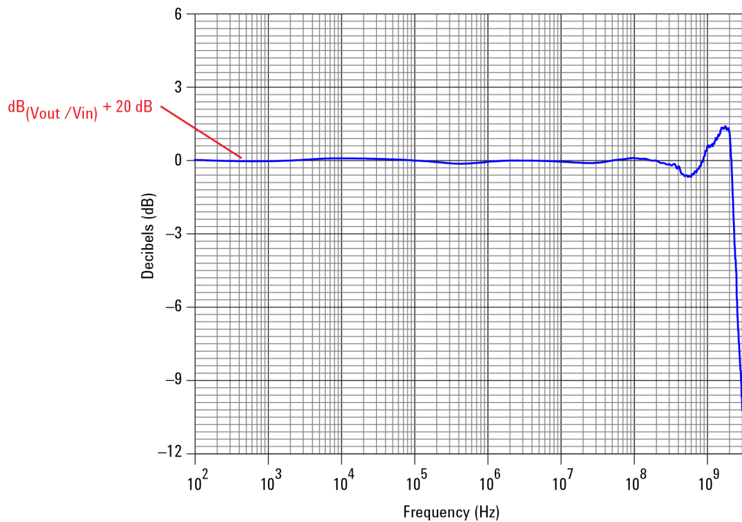
Figure 13 Frequency Response ( V_{\text{out}}/V_{\text{in}} )
