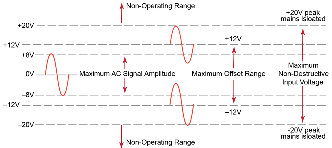
Figure 10 Dynamic Range and Offset Limits (mains isolated)
