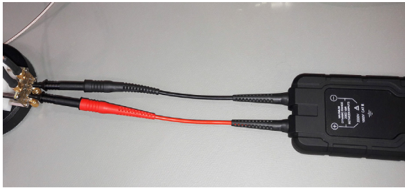
Figure 6 DP0001A Input leads running in parallel (Best case)
