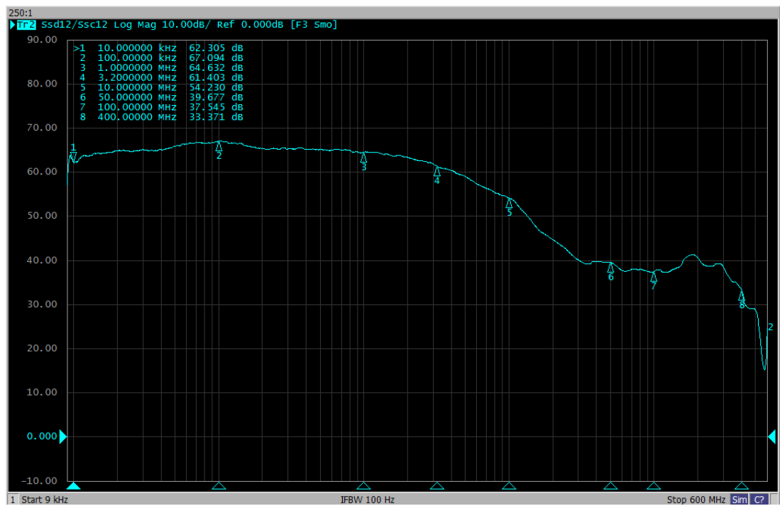
Figure 10 CMRR plot at 250:1
