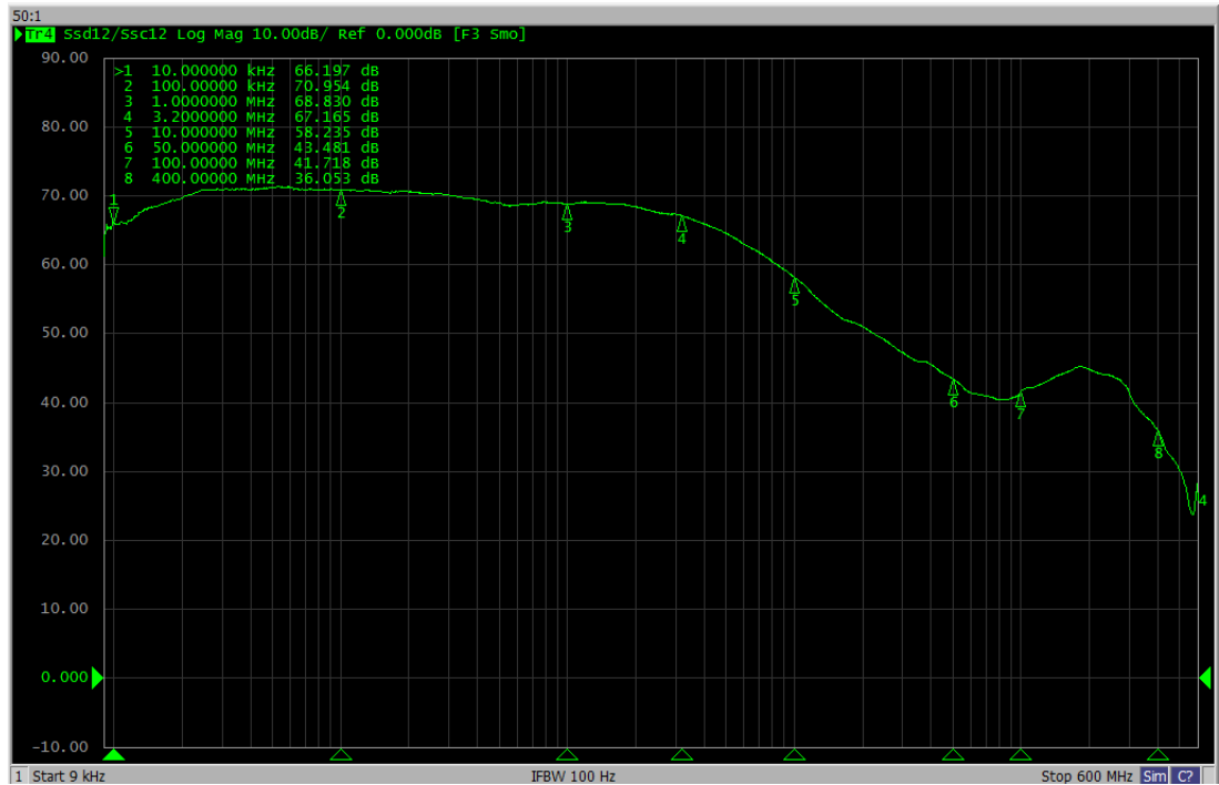
Figure 8 CMRR plot at 50:1
