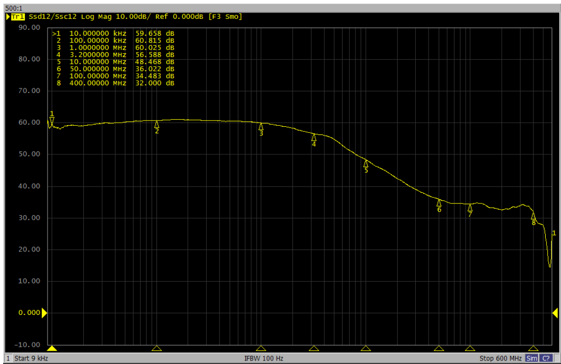
Figure 11 CMRR plot at 500:1
